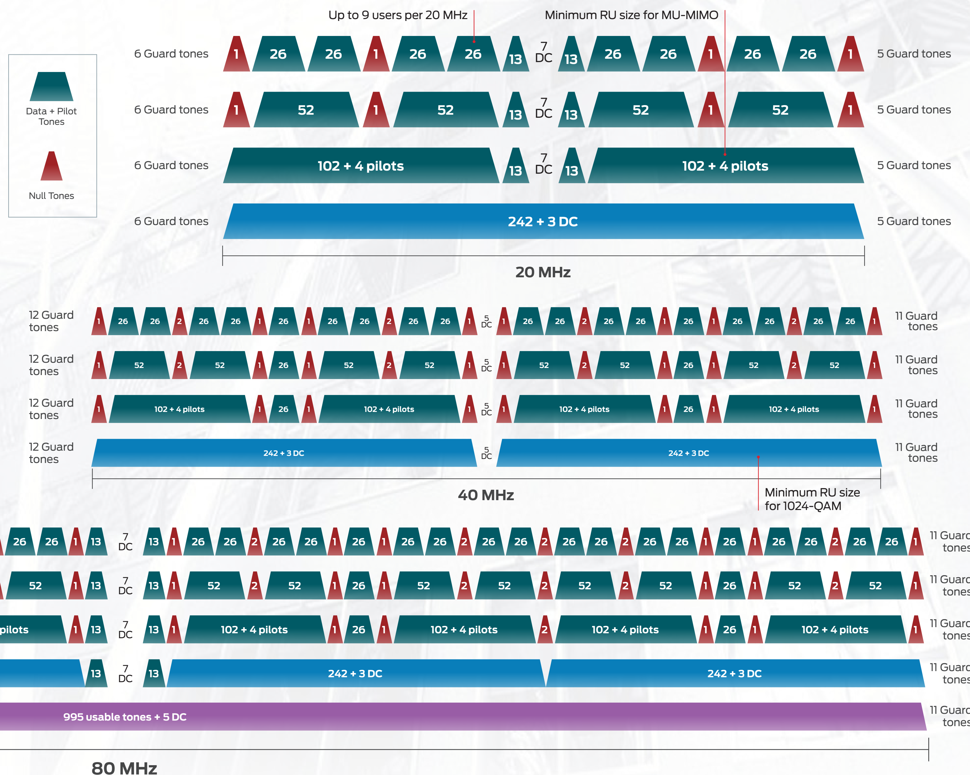
Resource Units and Channel Bandwidth
