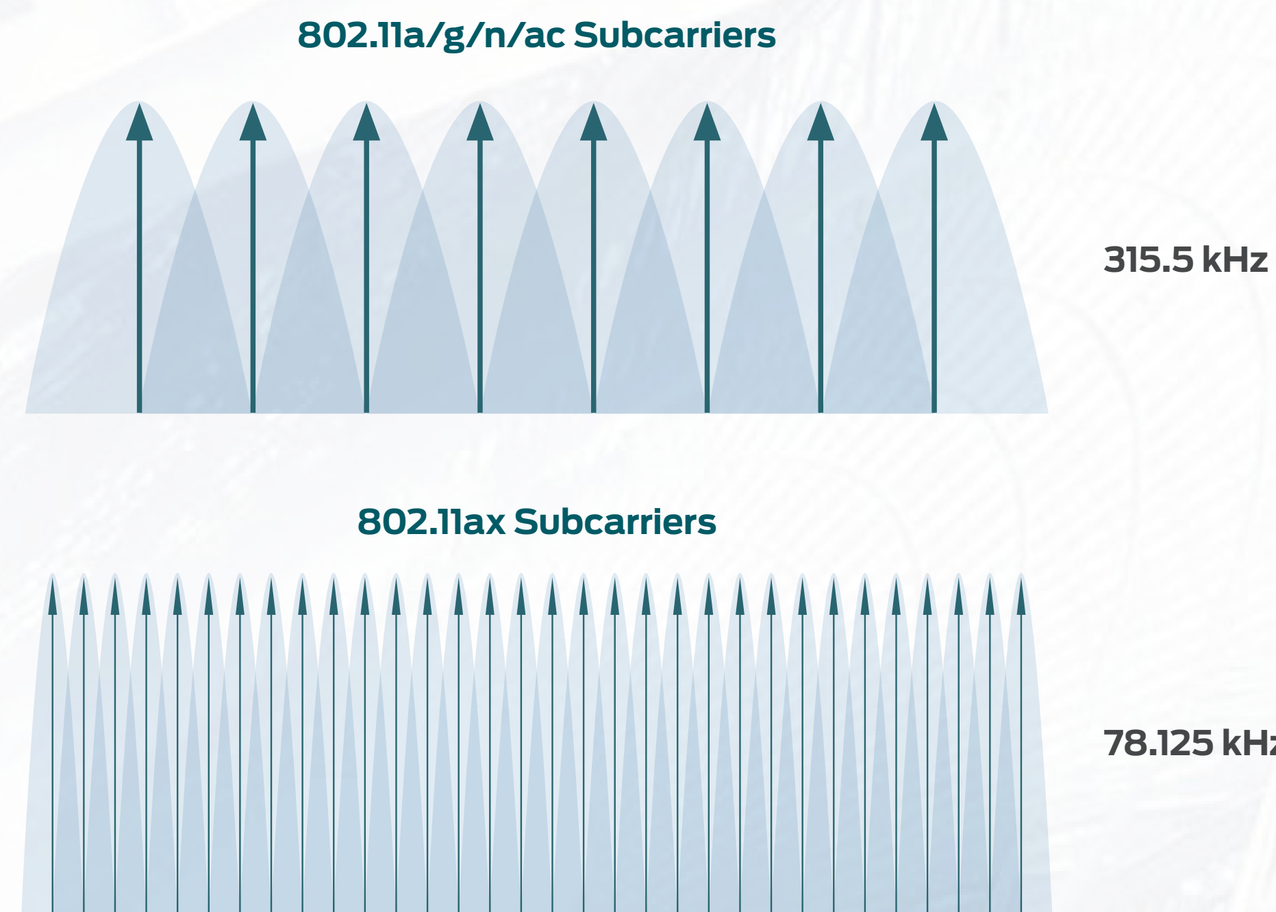
OFDM and OFDMA Subcarriers
