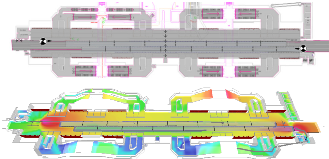
Figure 12: GSM coverage at platform 1 with two trains at the platform
