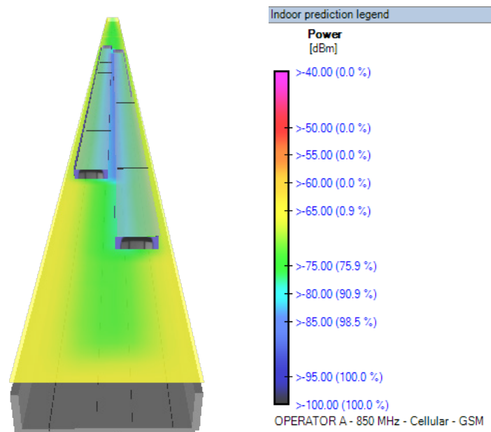
Figure 11: GSM coverage in a tunnel and inside trains (radiating cables at both walls)
