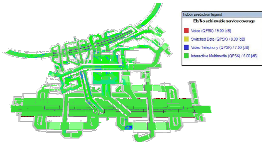
Figure 10: E_b/N_0 Coverage Map Used for Voice Sizing Example
